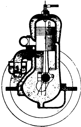
SECTION FERRO TWO-CYCLE MOTOR.
